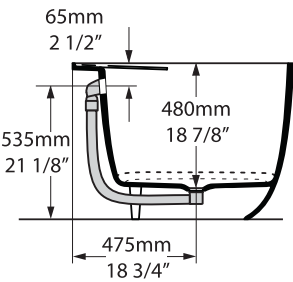
Section BB Shown with K60/K61 waste kit
